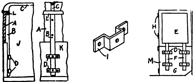
Fig. 1—Detail drawing of inside door, window attachment, etc.
